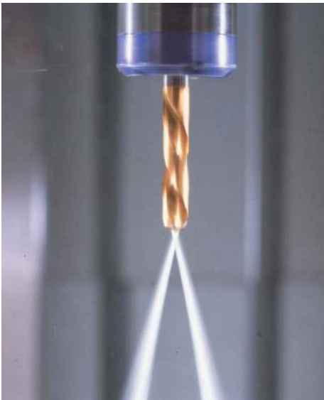
Coolant Through Spindle
