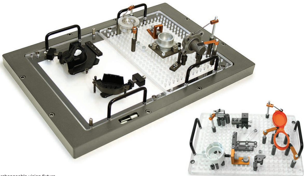
Interchangeable vision fixture
